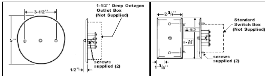
Model RL-HC [Ceiling]
